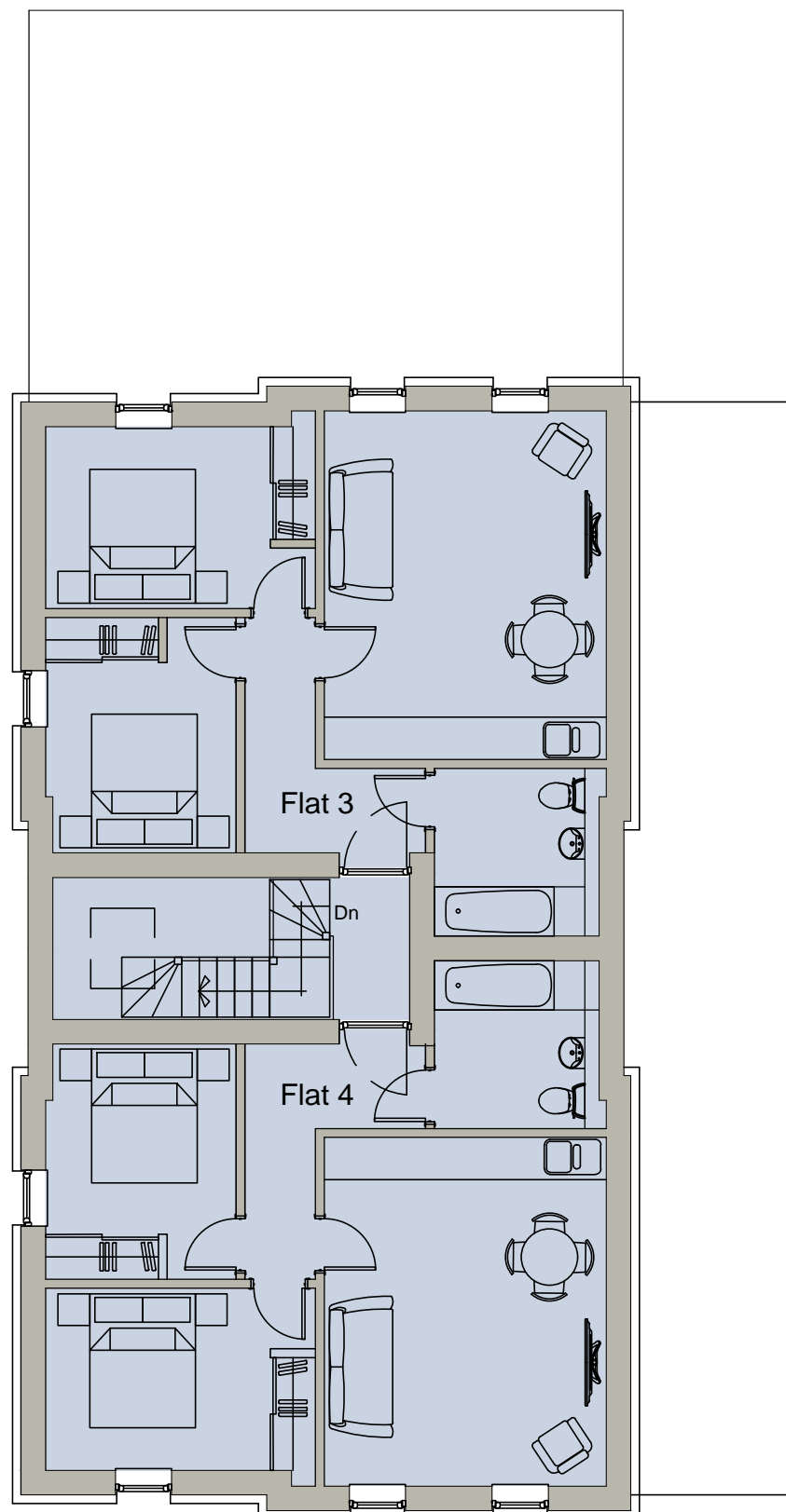
First Floor
